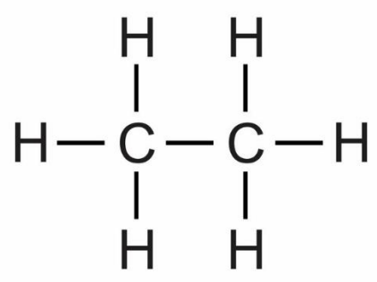
ETHANE
